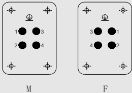
面板安装开孔图 Panel cut out for inserts for use without Hoods/housings
