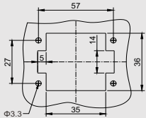
面板安装开孔图 Panel cut out for inserts for use without Hoods/housings
