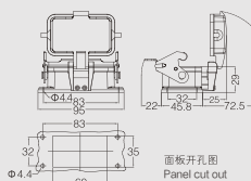
面板开孔图 Panel cut out
