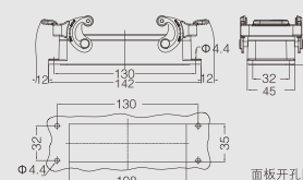
面板开孔图 Panel cut out
