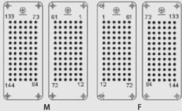
接插针排序 Contacts arrangement view from termination side
