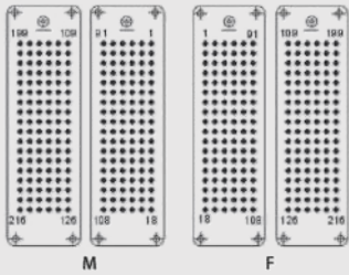
接插针排序 Contacts arrangement view from termination side
