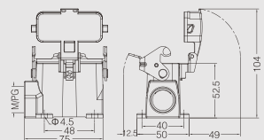
带保护盖With protection cover
