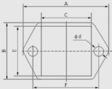
G3A开孔底座 G3A series housings
